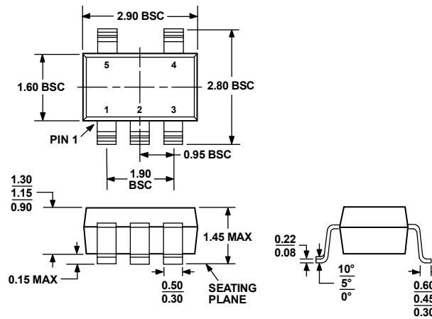
Figure 21. 5-Lead Small Outline Transistor Package [SOT-23] (RJ-5) Dimensions shown in millimeters
