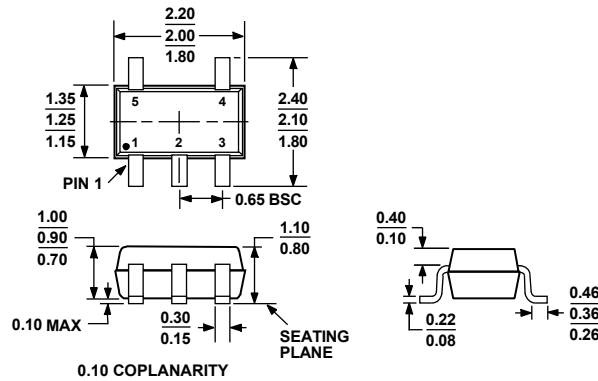
Figure 20. 5-Lead Thin Shrink Small Outline Transistor Package [SC70] (KS-5) Dimensions shown in millimeters
